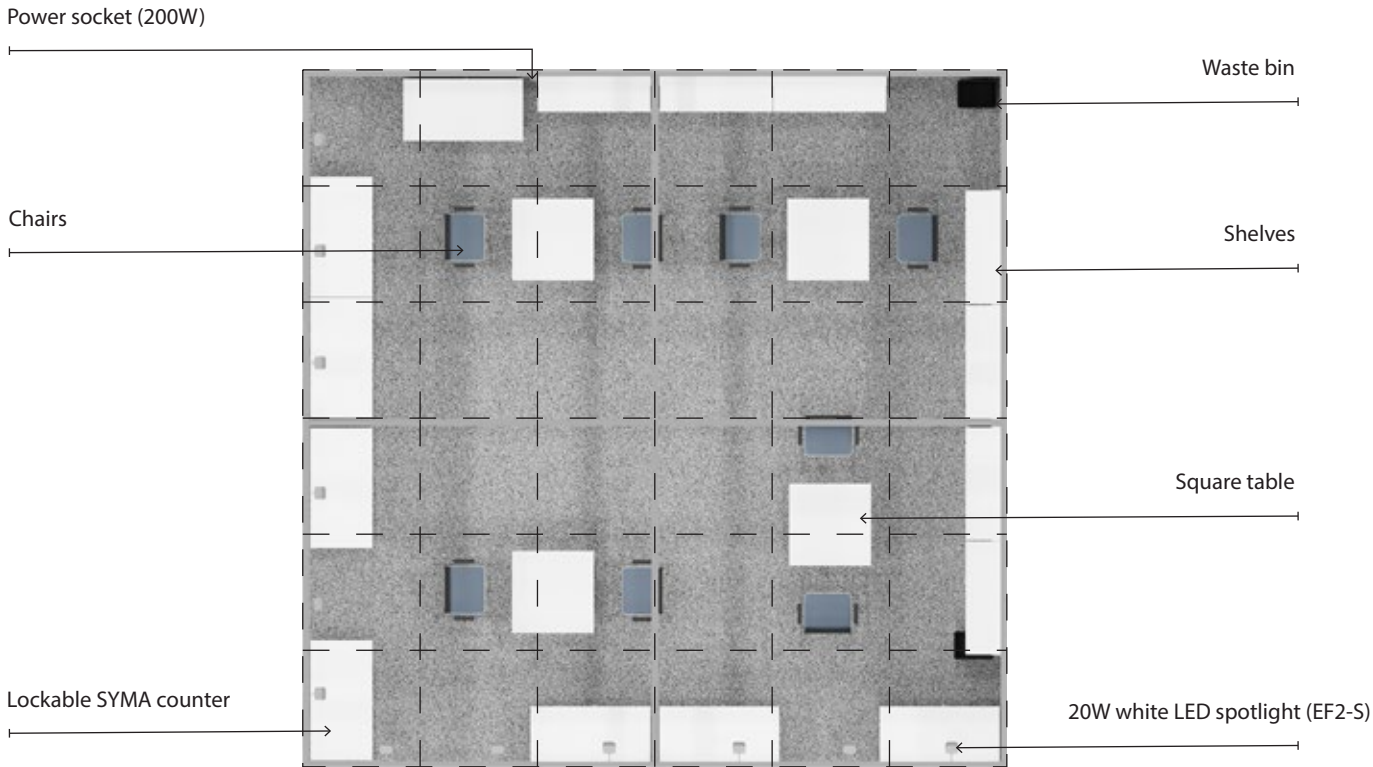
PLAN LAYOUT 2 SIDE OPEN
