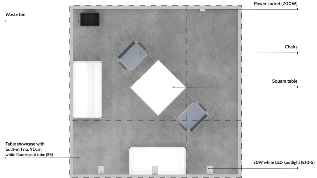
1 SIDE OPEN
